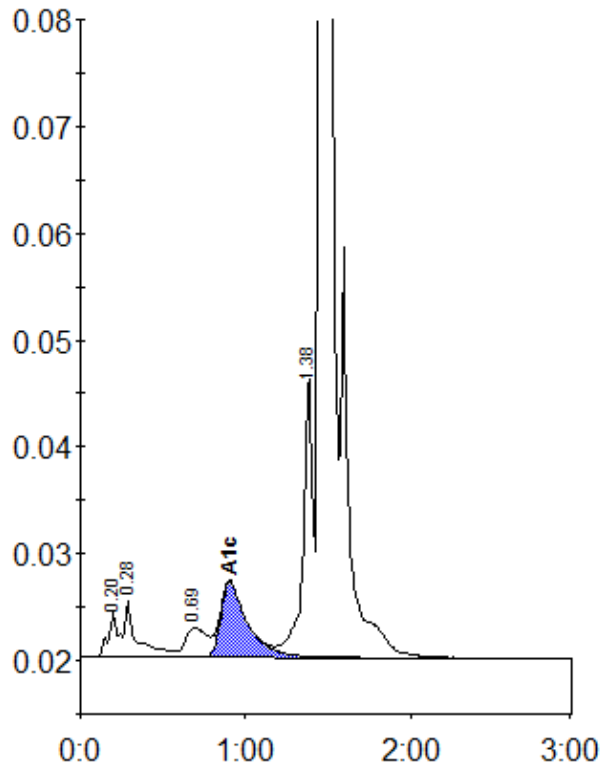
Peak table - ID: 10338587
